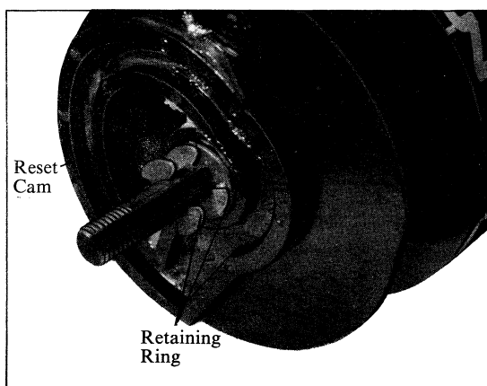
Figure 15. Reset Cam Removal.
