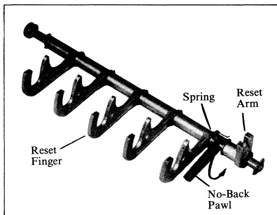
Figure 20. Reset Finger Shaft Group Preparation For Installation.
