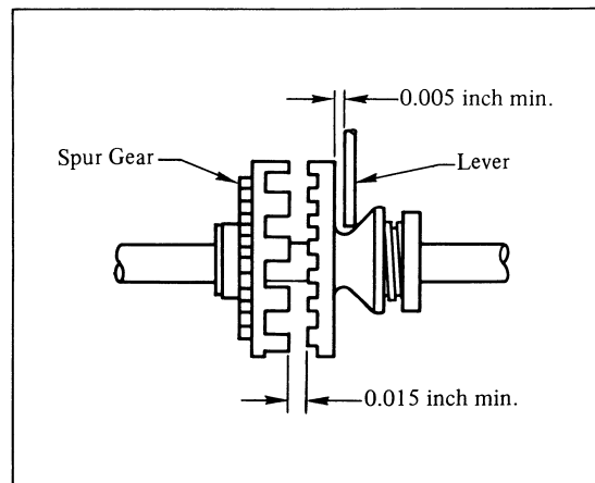
Figure 29. Clutch Lever Adjustment.
