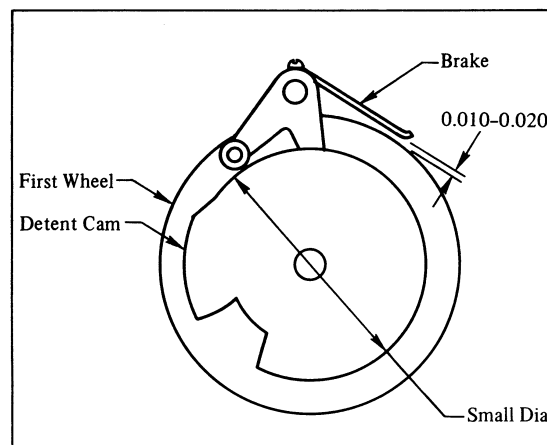
Figure 30. Brake Adjustment.
