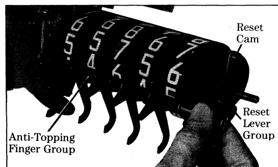
Figure 11. Anti-Topping Finger Group Removal.
