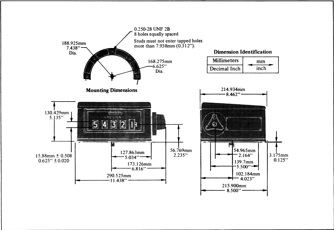
Figure 2. Mounting Dimensions — Series 7887 Meter Register.
