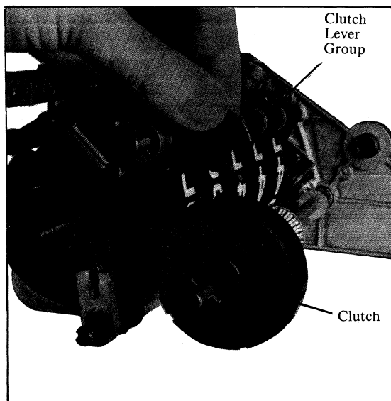
Figure 9. Clutch Group Removal
