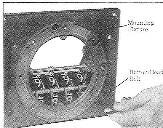
Figure 27. Securing Mounting Fixture.
