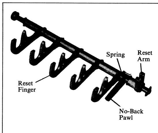
Figure 13. Reset Finger Group.
