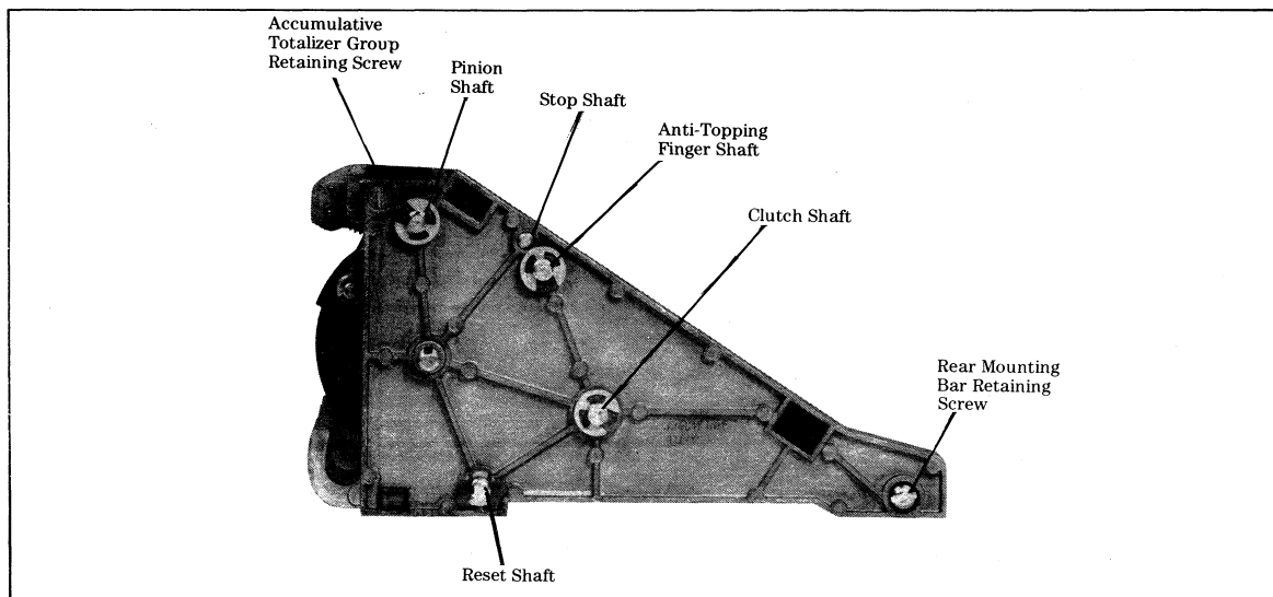
Figure 7. Right-Hand Side Plate.
