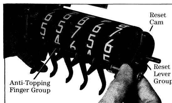
Figure 19. Anti-Topping Finger Group Installation.
