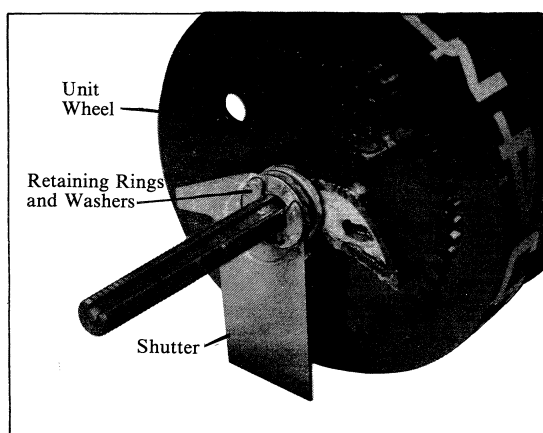
Figure 16. Unit Wheel Removal.
