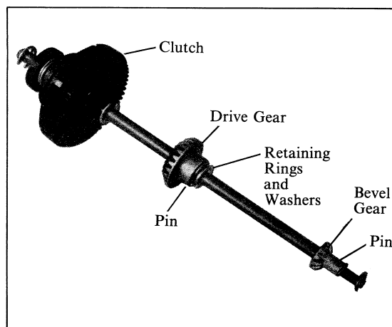
Figure 12. Clutch Shaft Group.
