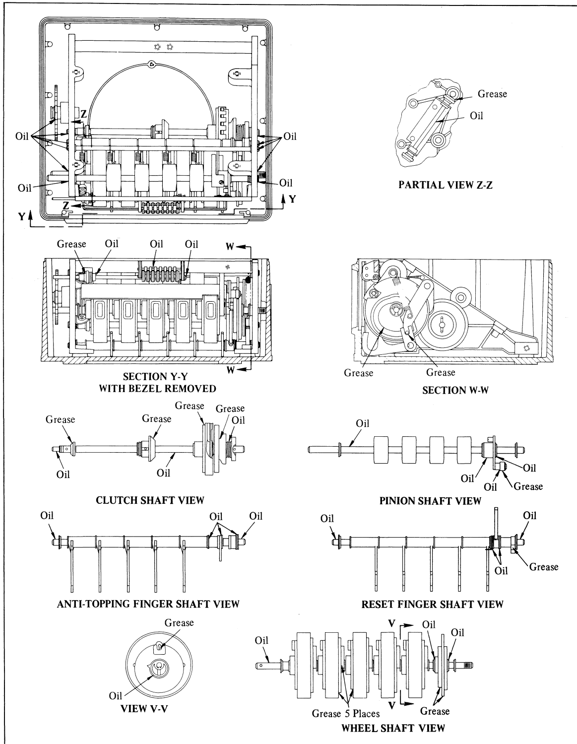
Figure 6. Lubrication Points.
