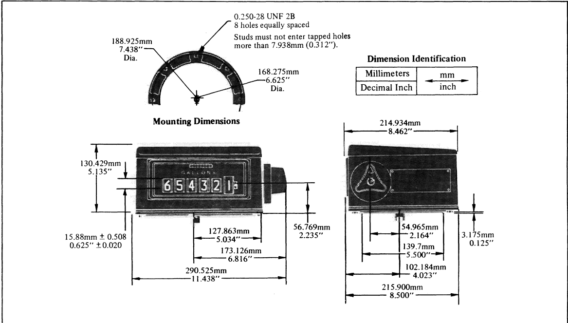
Figure 4. Mounting Dimensions — Series 7886 High-Capacity Meter Register.
