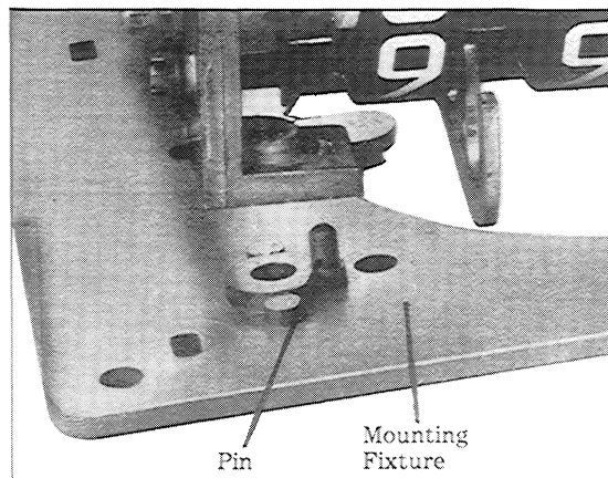
Figure 26. Installation Of Meter Register Onto Mounting Fixture.
