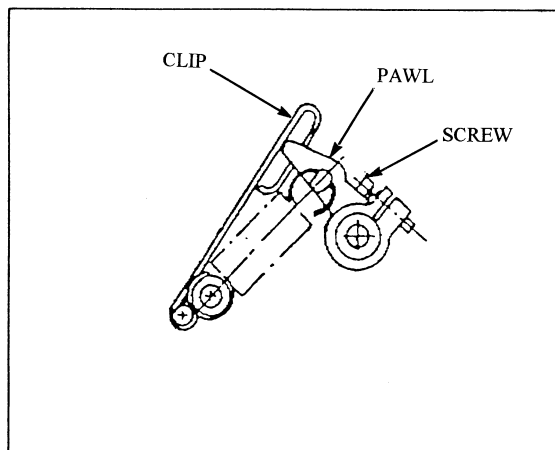
Figure 32. Backlash Compensating Mechanism (EEC UNITS)
