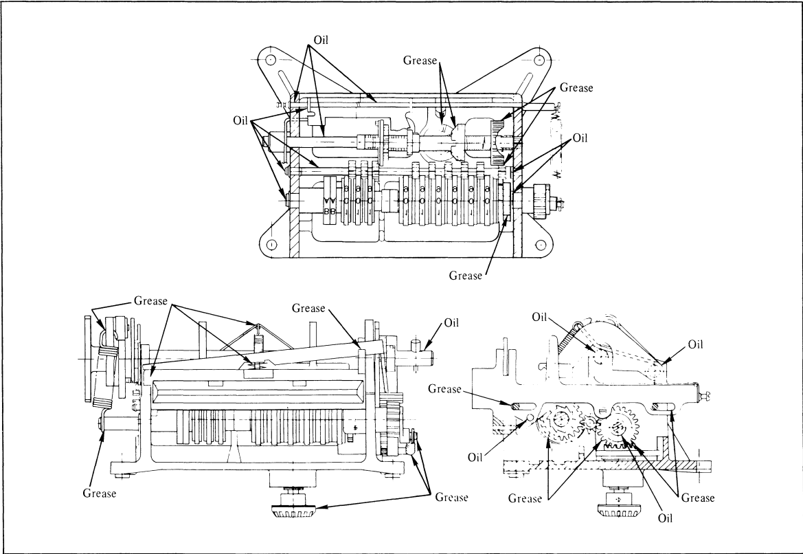
Figure 8. Lubrication Points - Zero Start Printer
