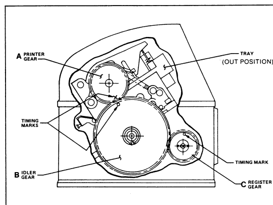
Figure 6. Assembling Printer to Meter Register
