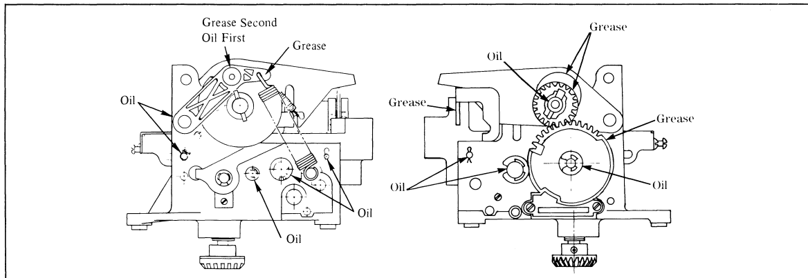
Figure 9. Lubrication Points - Accumulative Printer
