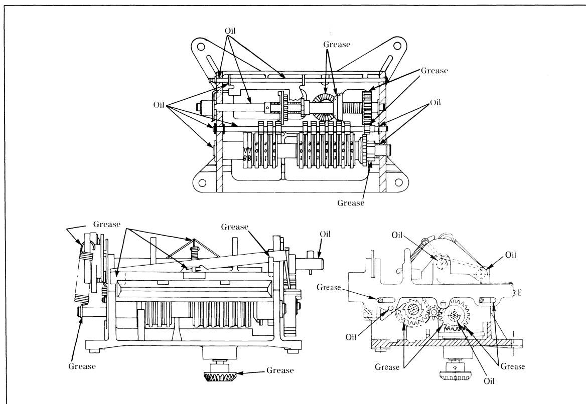
Figure 10. Lubrication Points - Accumulative Printer
