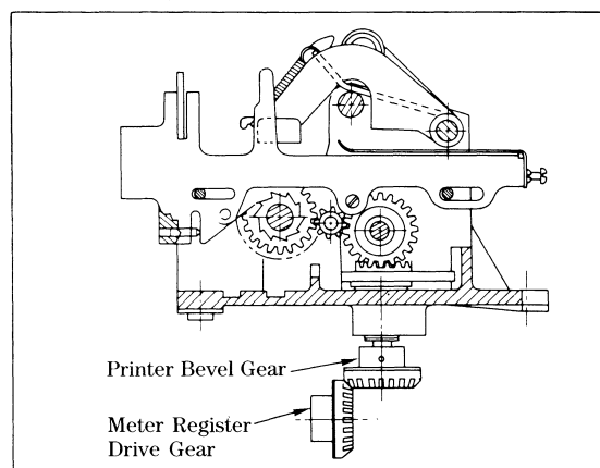
Figure 20. Ticket Printer/Meter Register Backlash Adjustment.
