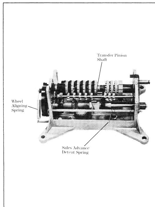
Figure 15. Sales Advance Mechanism
