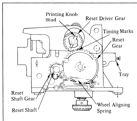
Figure 3. Reset Train (Zero Start)
