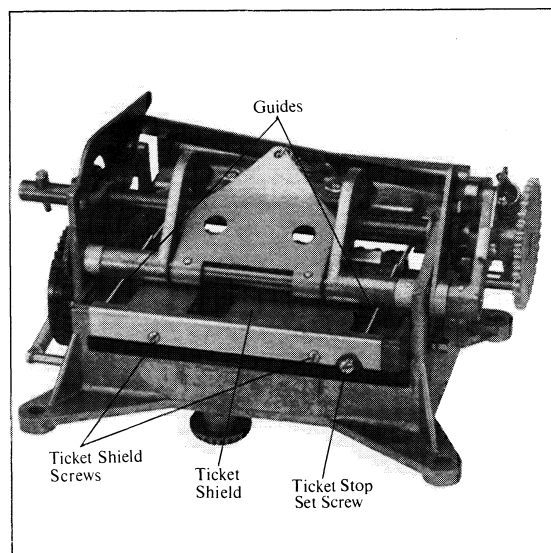
Figure 16. Ticket Position Guides and Stop Screws
