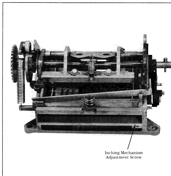
Figure 18. Right-Hand Wheel Inching Mechanism Adjustment Screw
