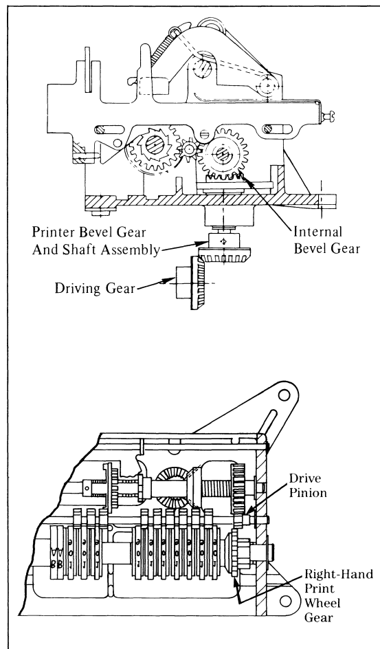
Figure 4. Drive Train (Accumulative)
