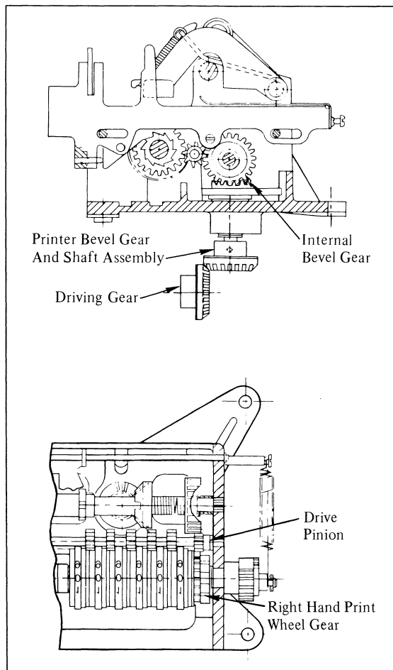
Figure 2. Drive Train (Zero Start)
