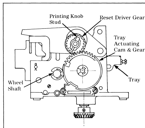
Figure 5. Tray Actuating Train (Accumulative)
